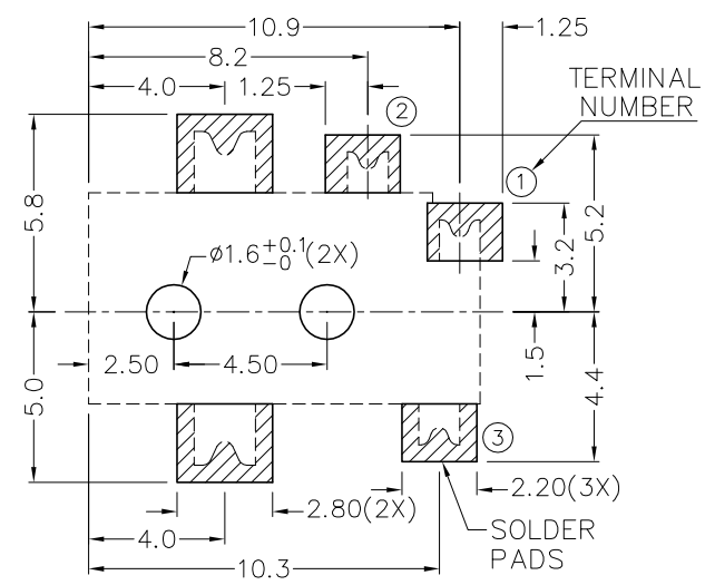
RECOMMENDED SOLDER PAD LAYOUT (TOP VIEW)
