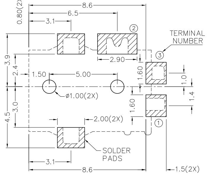
RECOMMENDED SOLDER PAD LAYOUT (TOP VIEW)
