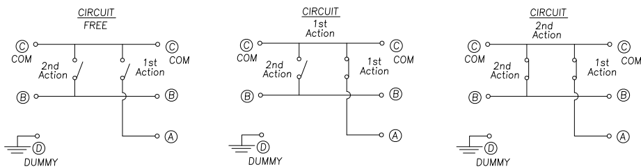
CIRCUIT DIAGRAM
